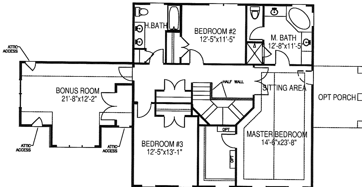
Davenport Second Floor Plan-Craftsman
