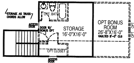
Nantahala Second Floor Plan-Lodge
