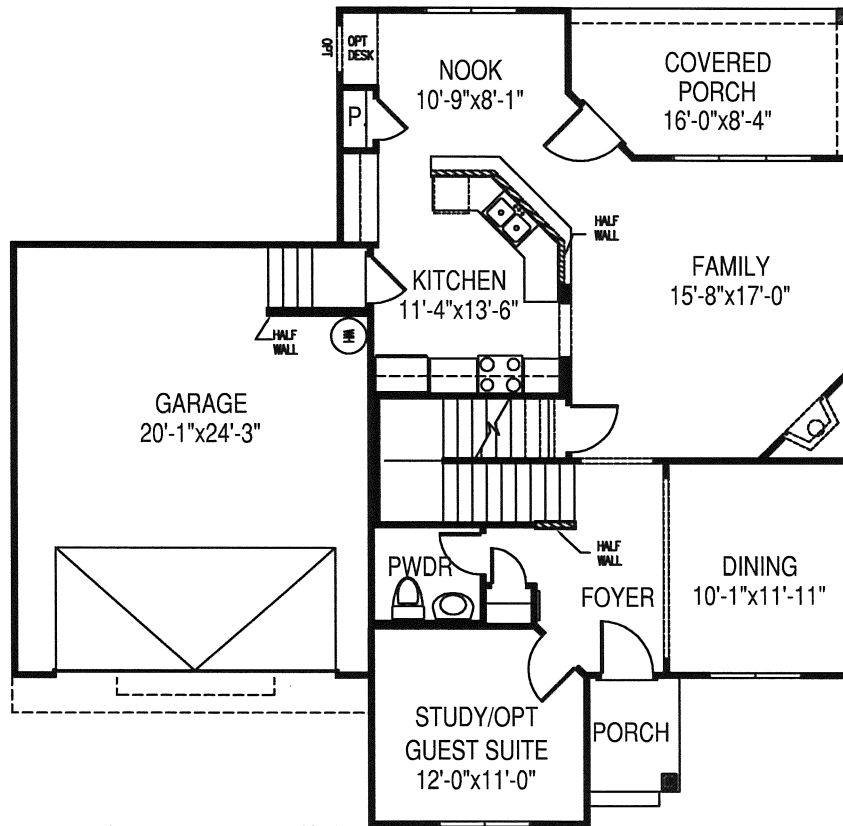
Chattooga English First Floor Plan
